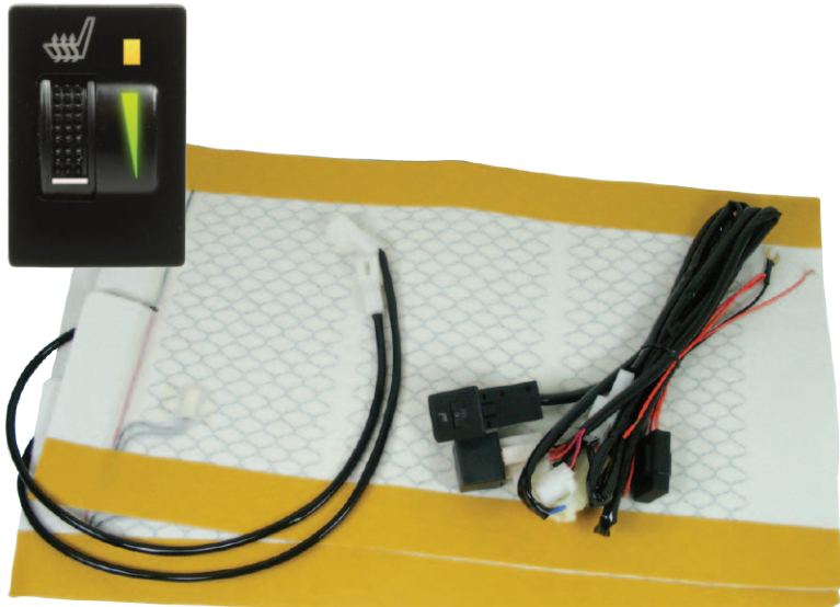
Seat heating system for one seat. Toyota-specific.
